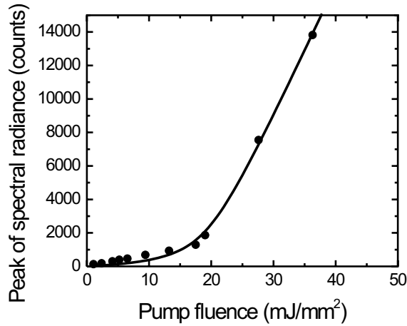
FIG. 4. Peak of the measured spectral radiance vs pump fluence for a random laser pumped with picosecond pulses. The solid line is a fit to our data, with the parameters \tau=3200 ps and the mean cavity decay time 0.1 ps. From the fit we obtain \beta_{\text{eff}}=0.03 [Eq. (16)].
