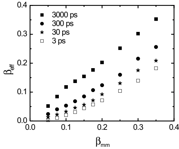
FIG. 2. The theoretical values of the effective \beta factor, \beta_{\text{eff}} , numerically calculated from the rate equations, vs the input parameter \beta_{\text{mm}} for different pump pulse durations. We choose the input parameters relevant for our experiments: \tau=3200 ps and \tau_c=0.1 ps. In the legend the pump pulse durations are listed.
