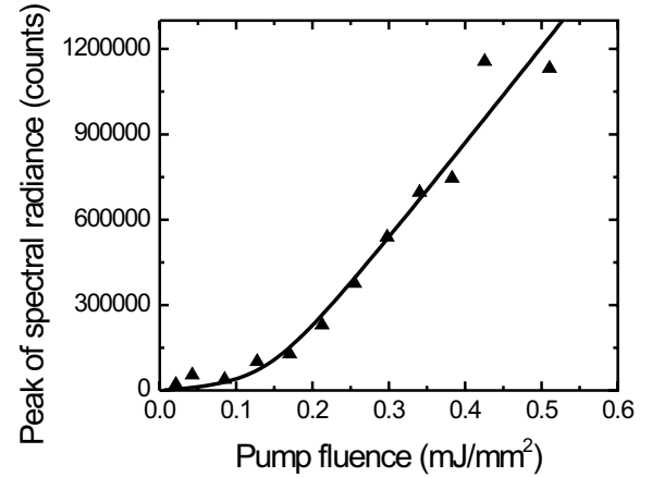
FIG. 3. Peak of the measured spectral radiance of the random laser vs the pump fluence for a random laser pumped with nanosecond pulses. A normal threshold behavior is observed. The solid line is a fit to our data, with \tau_{c,\text{mm}}=0.1 ps, and the spontaneous emission lifetime is 3200 ps. From the fit we obtain \beta_{\text{eff}} = 0.07 , which in our model equals the probability of lasing p_l [Eq. (16)].
