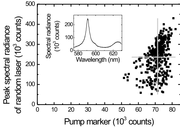
FIG. 1. The peak of the spectral radiance of the random laser is plotted vs the pump marker. The two gray lines indicate the mean values of the two peak heights and are used to visualize the correlation. The inset shows a typical single shot spectrum, from which the counts of the peak heights are determined.
