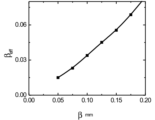
FIG. 5. The calculated \beta_{\text{eff}} vs the input parameter of the rate equations \beta_{\text{nm}} is shown. The graph is produced for a pump pulse duration of 15 ps, \tau_{c,\text{nm}}=0.1 ps, and \tau=3200 ps. The solid lines connect the data points. We convert our \beta_{\text{eff}} of 0.03 to a p_l of 0.09.
